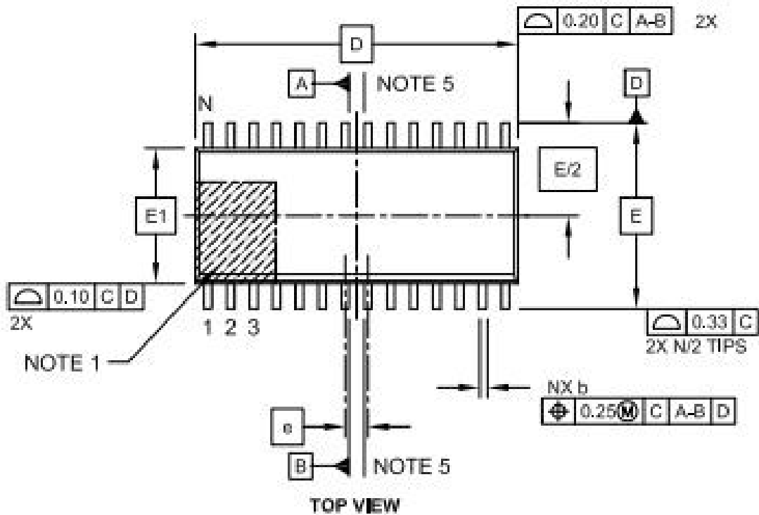
Typical 28-Lead Plastic Small Outline – Wide, 7.5 mm Body [SOIC]
